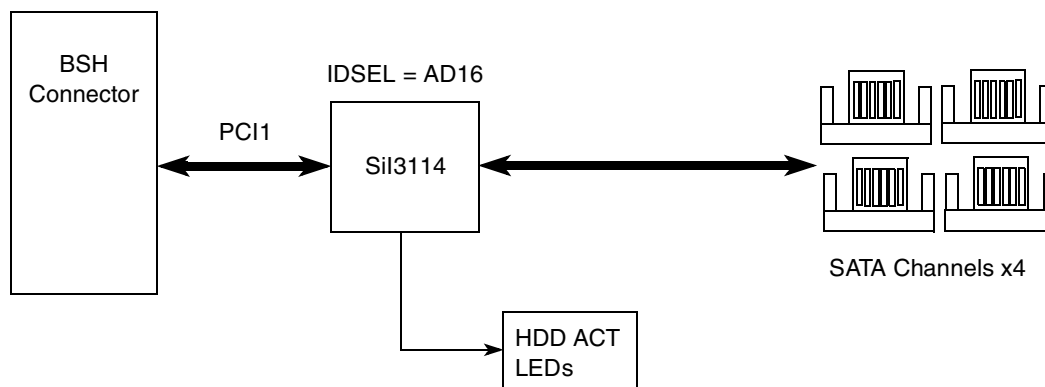
Figure 10. SiI3114 Connections
